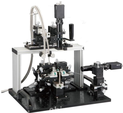
Fiber-Optic CCD Alignment System
